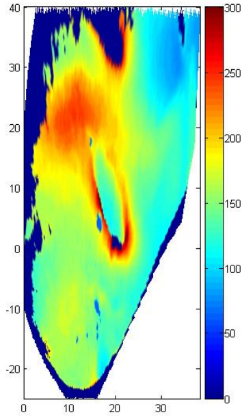
Fig 3.11: Top view of the Heat Transfer Contour showing the values of heat transfer coefficient in W/m^2-K . Color to heat transfer coefficient correlation is shown in the color scale from 0-300 W/m^2-K
