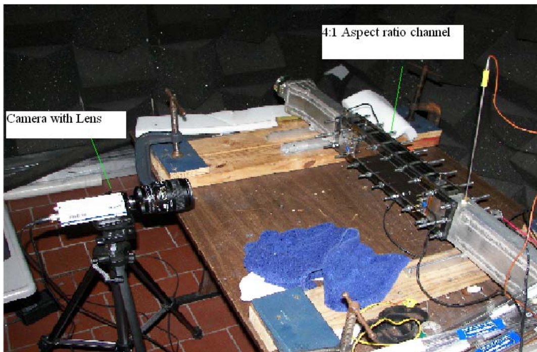
Fig 3.3: Experimental Setup for Benchmarking the Camera-Endoscope combination
